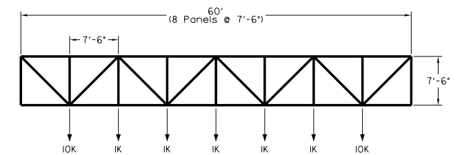
TRUSS T3
