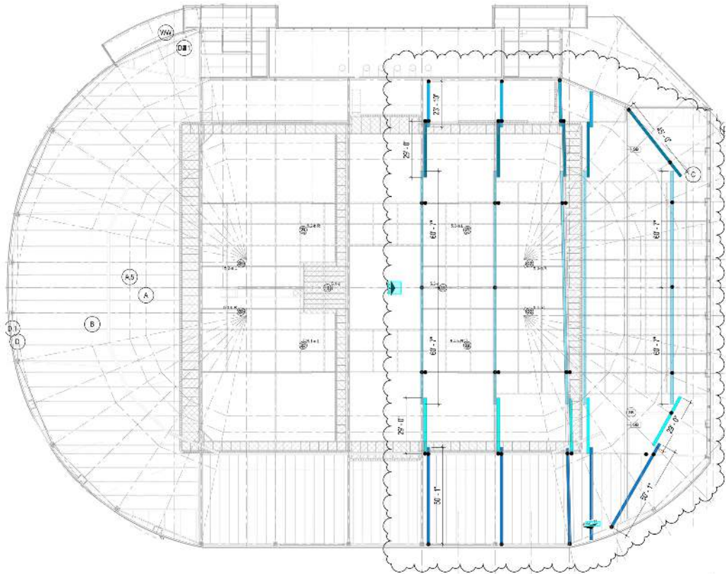
① HALF HOUSE REDUCTION CURTAINS -OVERALL RCP 182-1-F
