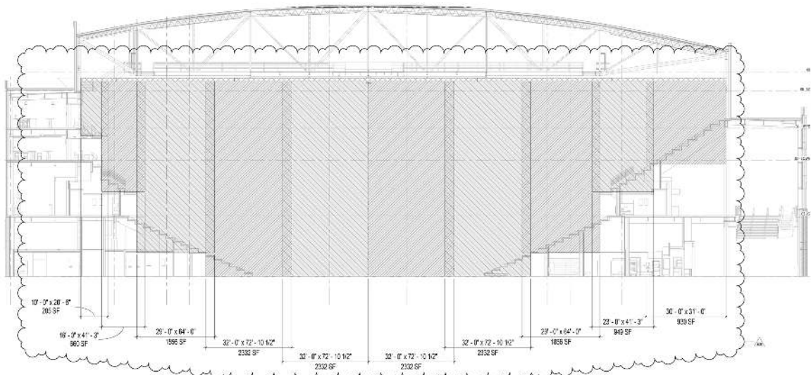
① HALF HOUSE REDUCTION CURTAINS - EAST ELEVATION 182-1-F
